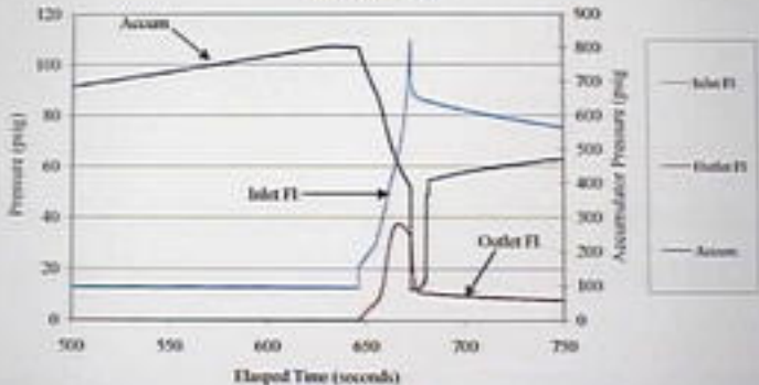
September 20, 2000 HP Exemplar Pilot Valve Run #2: Plot B
