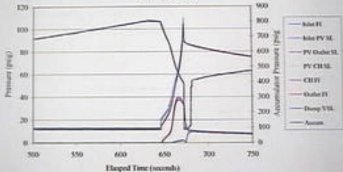
September 20, 2008 HP Exemplar Pilot Valve Run #2: Plot A
