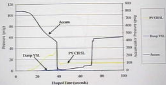
September 20, 2000 HP Exemplar Pilot Valve Run #1: Plot E
