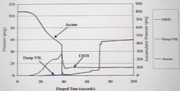
September 20, 2000 HP Exemplar Pilot Valve Run #1: Plot D
