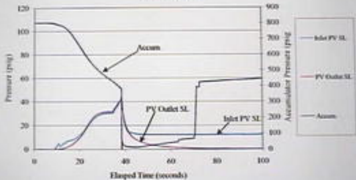
September 20, 2000 HP Exemplar Pilot Valve Run #1: Plot C
