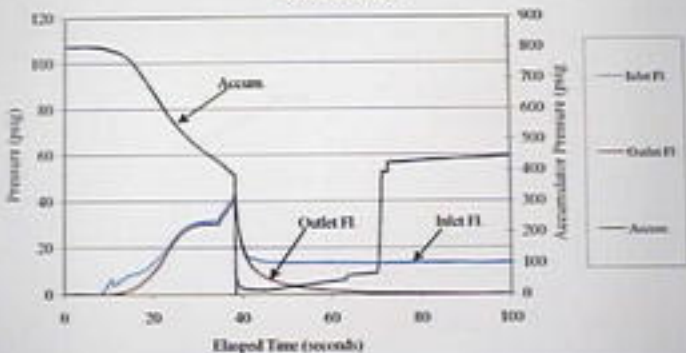
September 20, 2000 HP Exemplar Pilot Valve Run #1: Plot B
