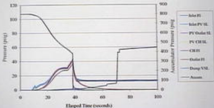
September 20, 2000 HP Exemplar Pilot Valve Run #1: Plot A
