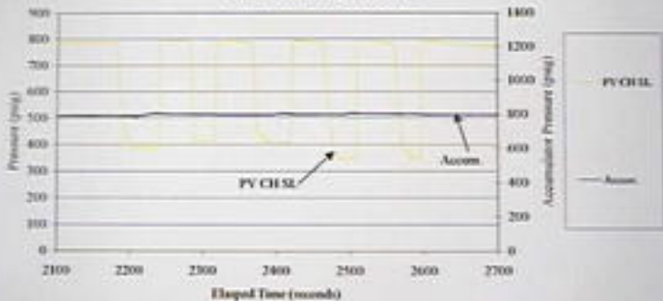
September 21, 2000 LP Exemplar Pilot Valve with Adjusted Set-Point Runs #10 through 14; Plot E
