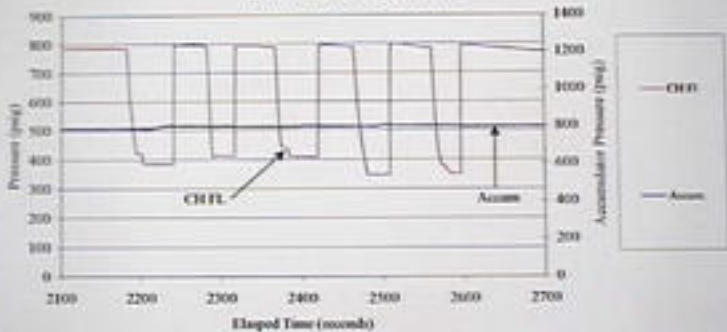
September 21, 2000 LP Exemplar Pilot Valve with Adjusted Set-Point Runs #10 through 14: Plot D
