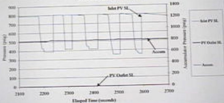
September 21, 2000 LP Exemplar Pilot Valve with Adjusted Set-Point Runs #10 through 14: Plot C
