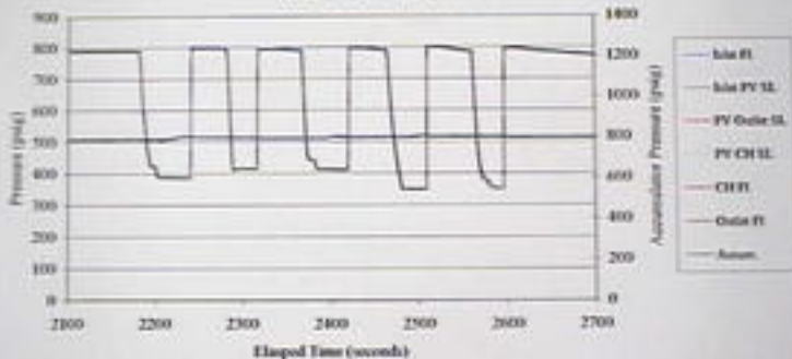
September 21, 2000 LP Exemplar Pilot Valve with Adjusted Set-Point Runs #10 through 14: Plot A
