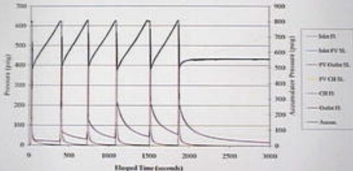
September 21, 2000 LP Exemplar Pilot Valve with Adjusted Set-Point Runs #1 through 6; Plot A
