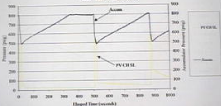
September 21, 2000 HEP Exemplar Pilot Valve Runs #1 through 3: Plot E
