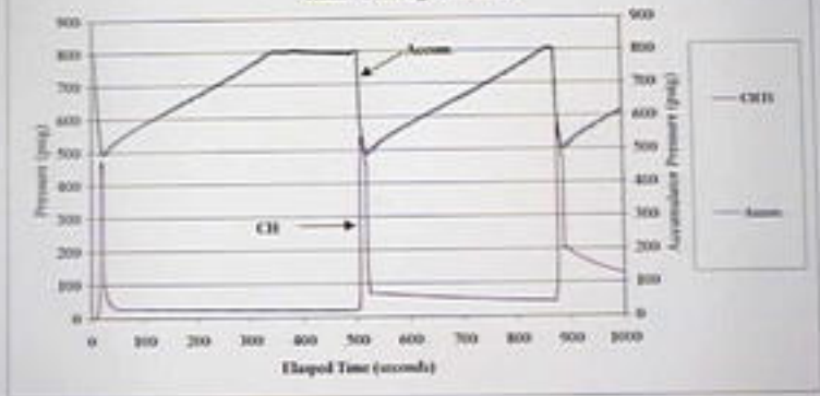
September 21, 2000 IIP Exemplar Pilot Valve Runs #1 through 3: Plot D
