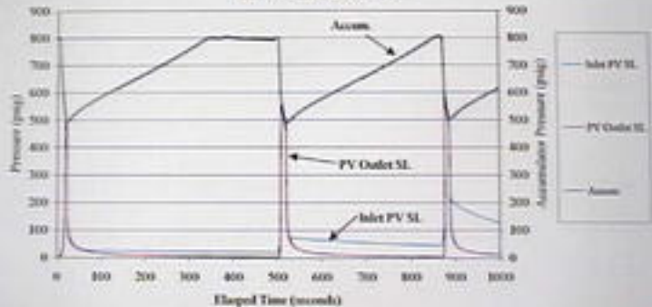
September 21, 2000 HP Exemplar Pilot Valve Runs #1 through 3: Plot C
