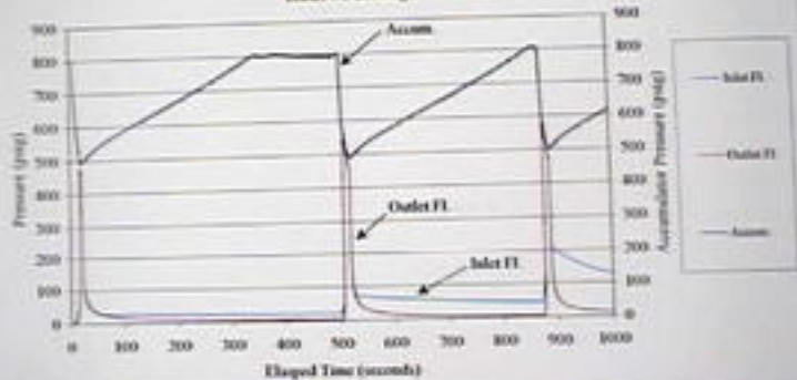
September 21, 2000 HP Exemplar Pilot Valve Runs #1 through 3: Plot B
