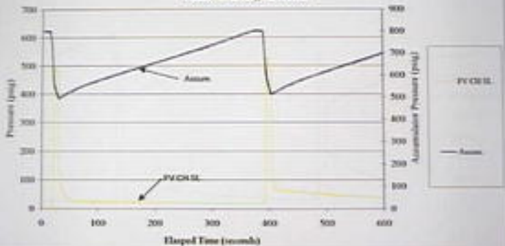
September 21, 2000 LP Exemplar Pilot Valve with Adjusted Set-Point Runs #1 through 2: Plot E
