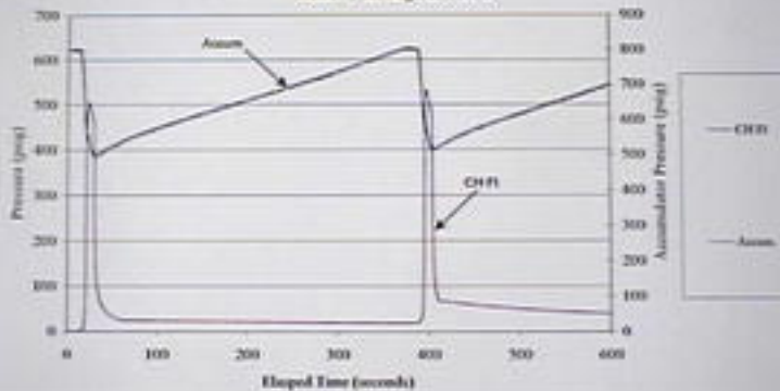
September 21, 2000 LP Exemplar Pilot Valve with Adjusted Set-Point Runs #1 through 2: Plot D
