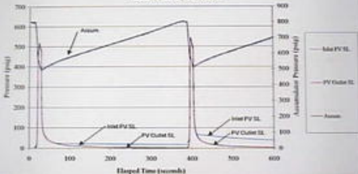
September 21, 2000 LP Exemplar Pilot Valve with Adjusted Set-Point Runs #1 through 2: Plot C
