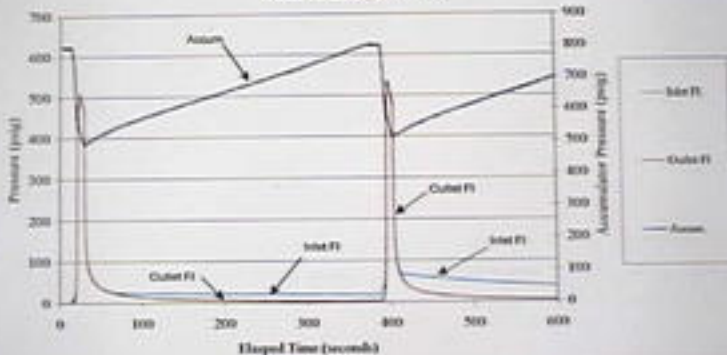
September 21, 2000 LP Exemplar Pilot Valve with Adjusted Set-Point Runs #1 through 2: Plot B
