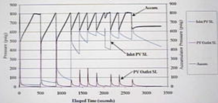
September 21, 2000 HP Exemplar Pilot Valve Runs #1 through 11: Plot C
