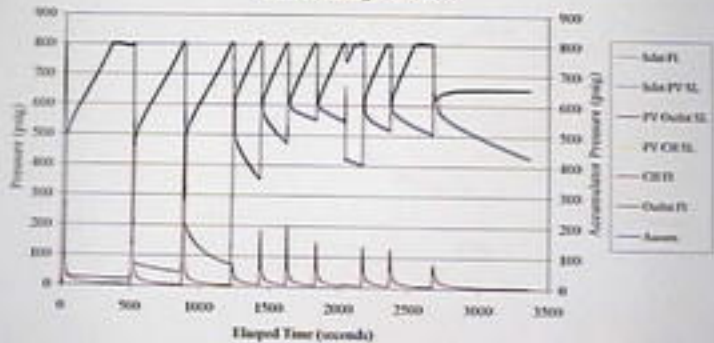
September 21, 2000 HP Exemplar Pilot Valve Runs #1 through 11: Plot A
