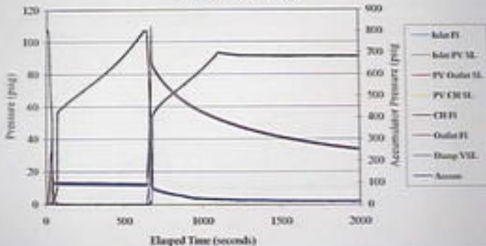
September 20, 2000 HP Exemplar Pilot Valve Runs #1 and 2: Plot A
