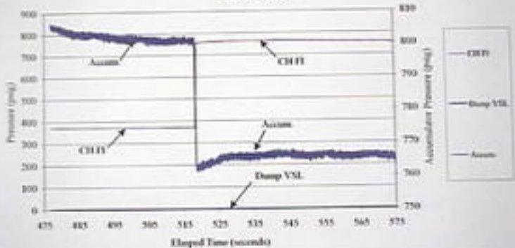
September 19, 2000 Accident Pilot Valve Run #6: Plot D
