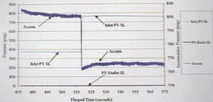
September 19, 2000 Accident Pilot Valve Run #6: Plot C
