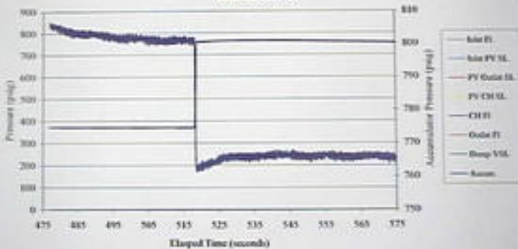
September 19, 2000 Accident Pilot Valve Run #6: Plot A
