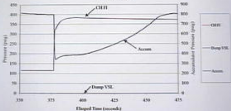
September 19, 2000 Accident Pilot Valve Run #5: Plot D
