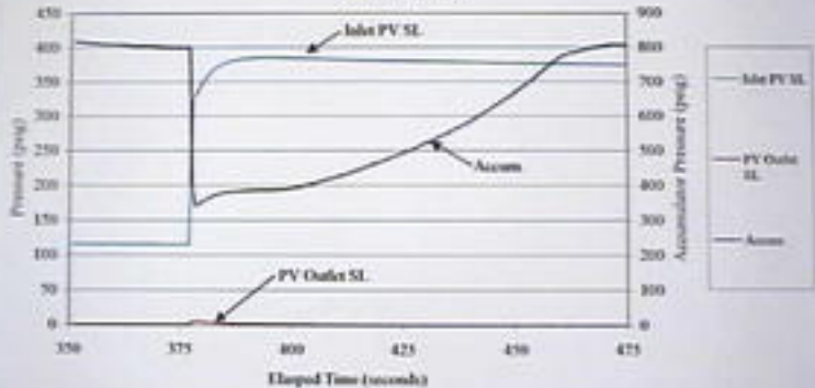
September 19, 2000 Accident Pilot Valve Run #5: Plot C
