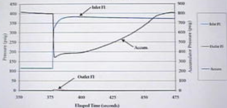
September 19, 2000 Accident Pilot Valve Run #5: Plot B
