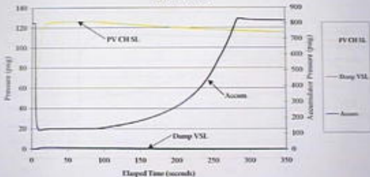
September 19, 2000 Accident Pilot Valve Run #4: Plot E
