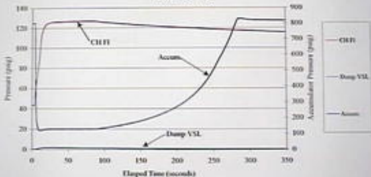
September 19, 2000 Accident Pilot Valve Run #4: Plot D
