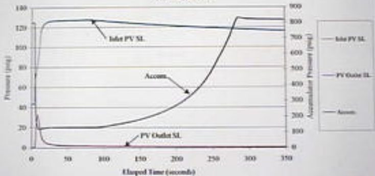
September 19, 2000 Accident Pilot Valve Run #4: Plot C
