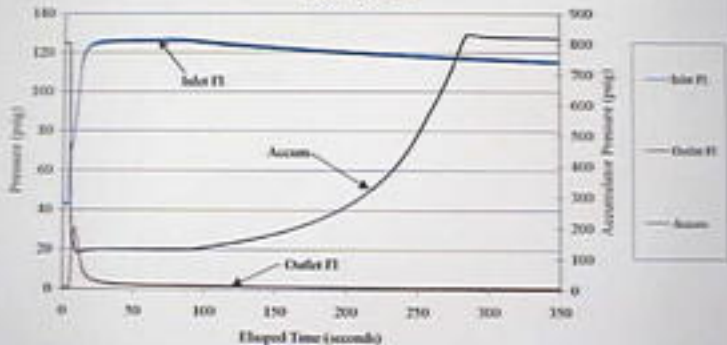
September 19, 2000 Accident Pilot Valve Run #4: Plot B
