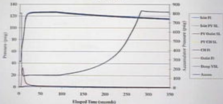
September 19, 2000 Accident Pilot Valve Run #4: Plot A
