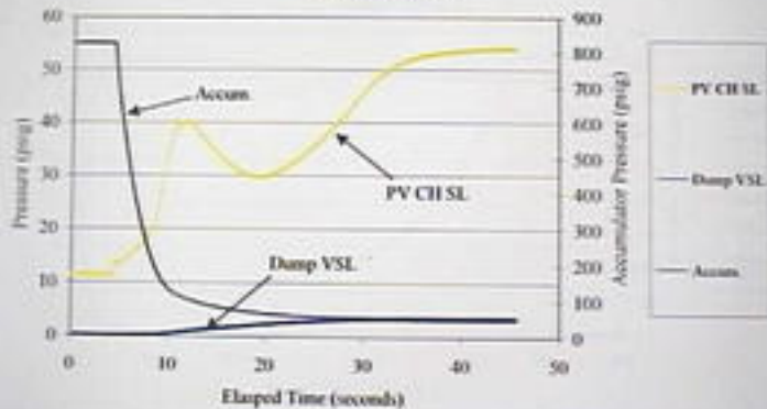
September 19, 2000 Accident Pilot Valve Run #3: Plot E
