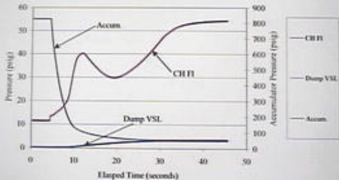
September 19, 2000 Accident Pilot Valve Run #3: Plot D
