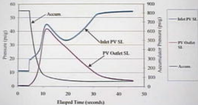
September 19, 2000 Accident Pilot Valve Run #3: Plot C
