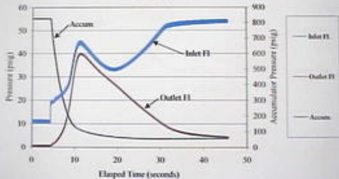
September 19, 2000 Accident Pilot Valve Run #3: Plot B
