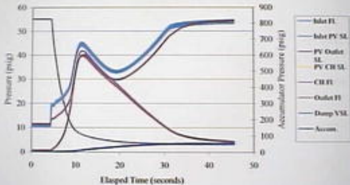
September 19, 2000 Accident Pilot Valve Run #3: Plot A
