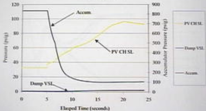
September 19, 2000 Accident Pilot Valve Run #2: Plot E
