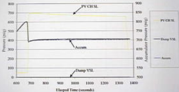
September 20, 2000 Accident Pilot Valve Run #2: Plot E
