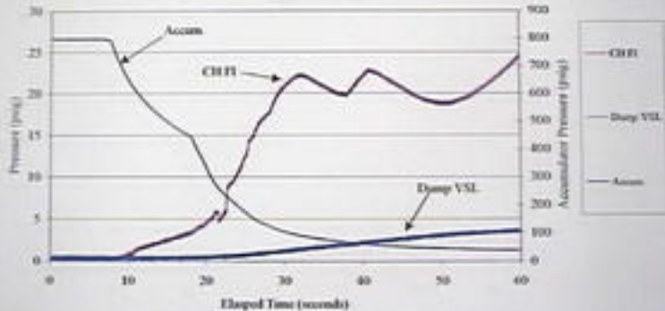
September 19, 2000 Accident Pilot Valve Run #1: Plot D2
