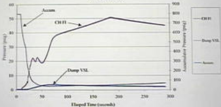
September 19, 2000 Accident Pilot Valve Run #1: Plot D
