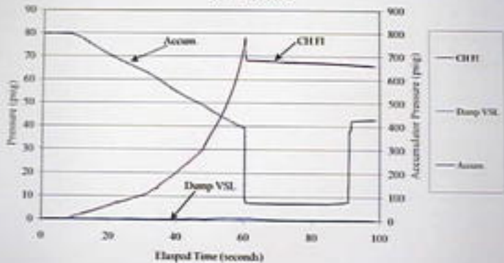
September 20, 2000 Accident Pilot Valve Run #1: Plot D
