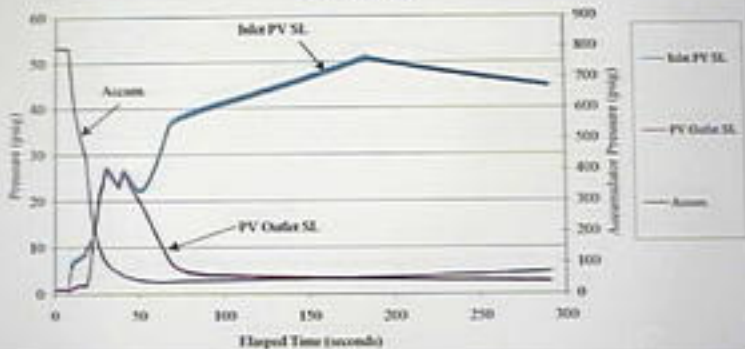
September 19, 2000 Accident Pilot Valve Run #1: Plot C
