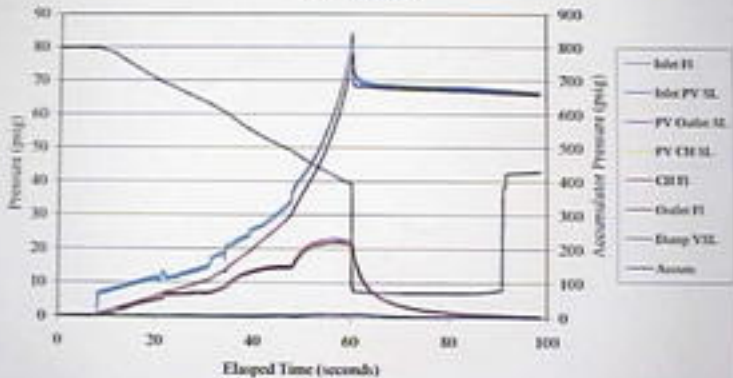
September 20, 2000 Accident Pilot Valve Run #1: Plot A
