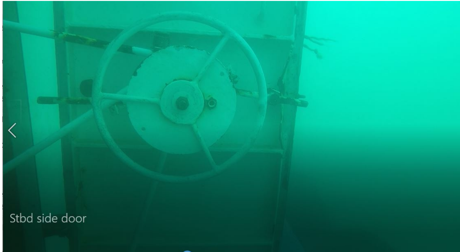
Proassist III starboard weathertight door
