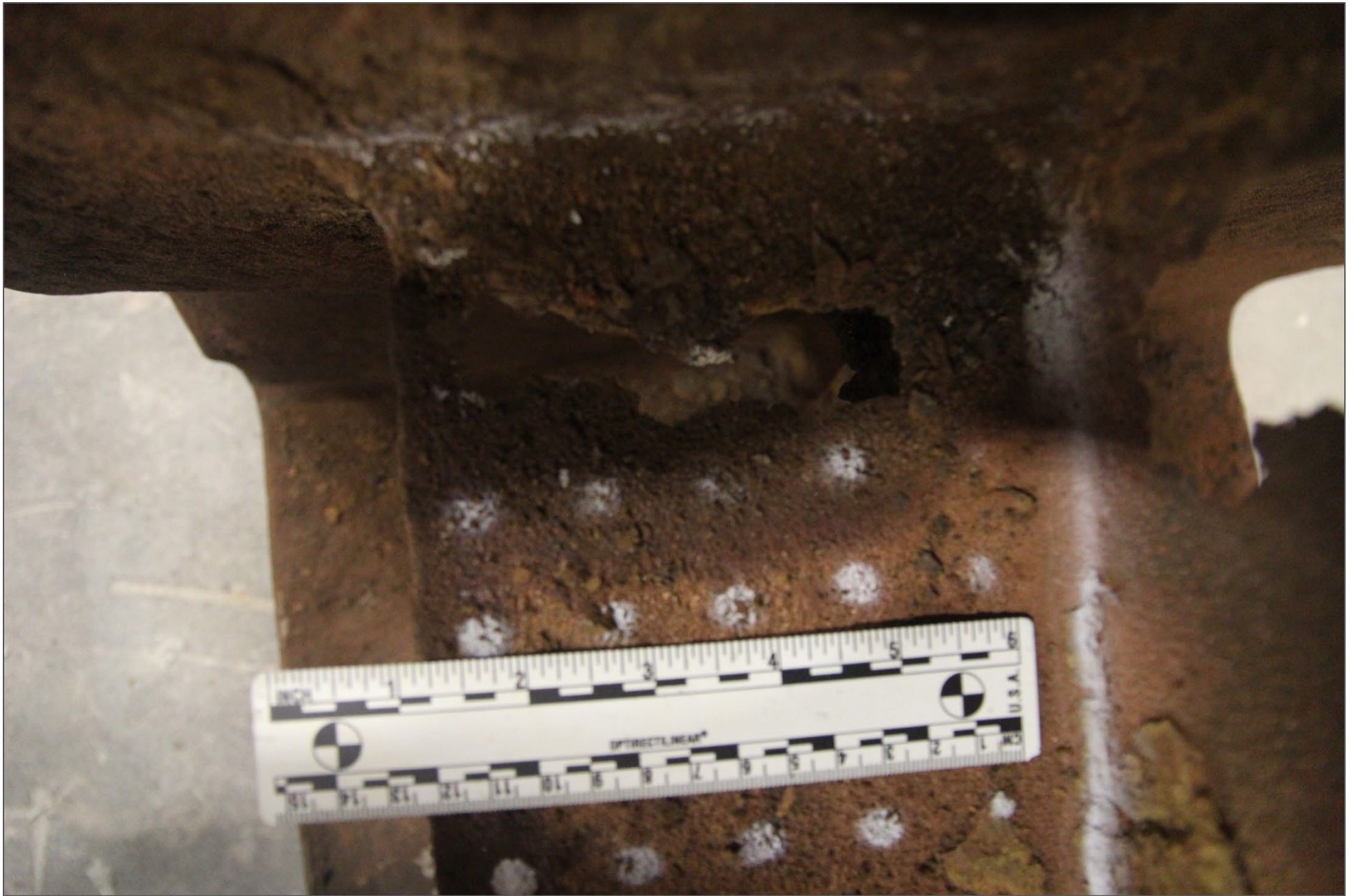
Materials Laboratory Photograph 8 – Closeup of Northwest Leg, Showing Longitudinal Stiffeners Just Above Transverse Tie Plate
