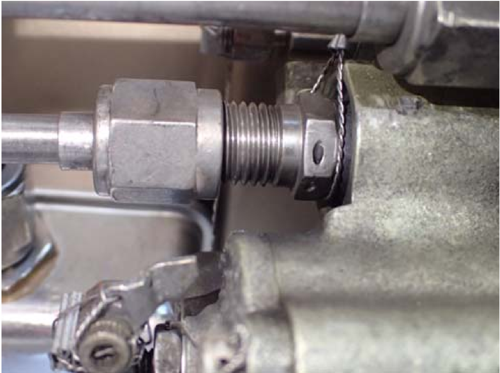
Photo 4 – View of the “B” nut at fuel control. (Photo courtesy of Rolls-Royce
