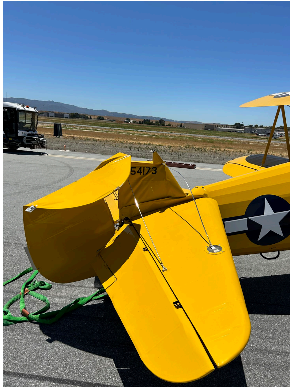
Photo 2 – Substantial damage to the vertical stabilizer and the rudder. Photo pilot.
